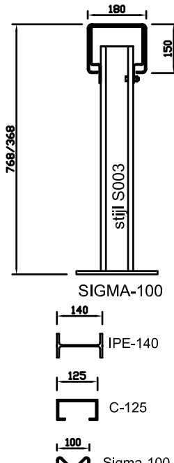
koker LS150/180
