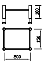
instort-anker
