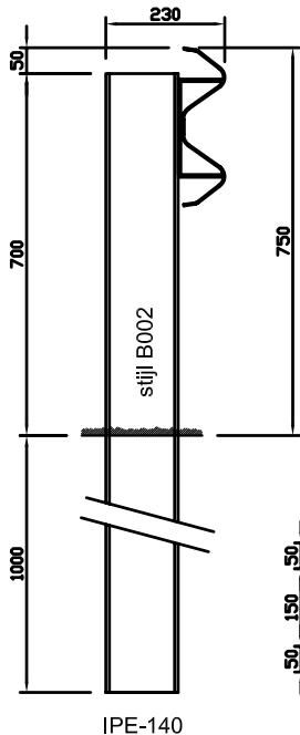
railprofiel A001
